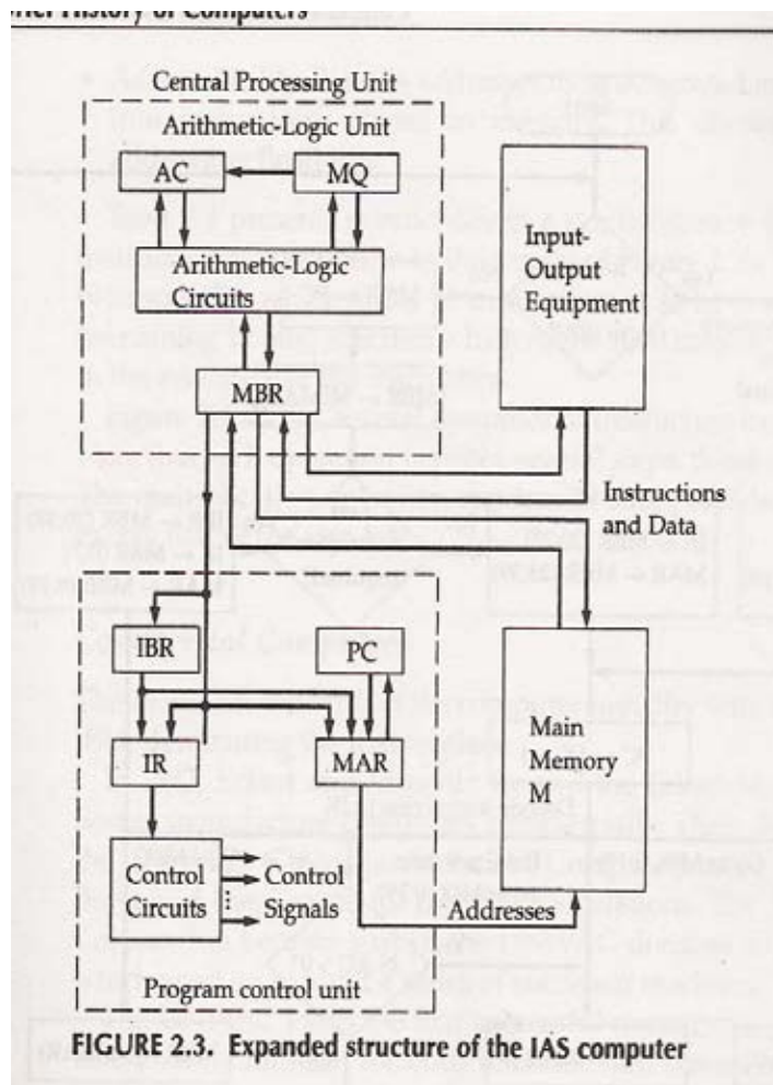
Fig Expanded structure of the IAS computer
